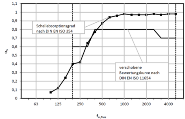
Mittenfrequenz Terz- / Oktavband f_{m, \text{Terz}} / f_{m, \text{Oktave}} in Hz Schallabsorptionsgrad je Terz- / Oktavband \alpha_{S, \text{Terz}} / \alpha_{S, \text{Oktave}}
